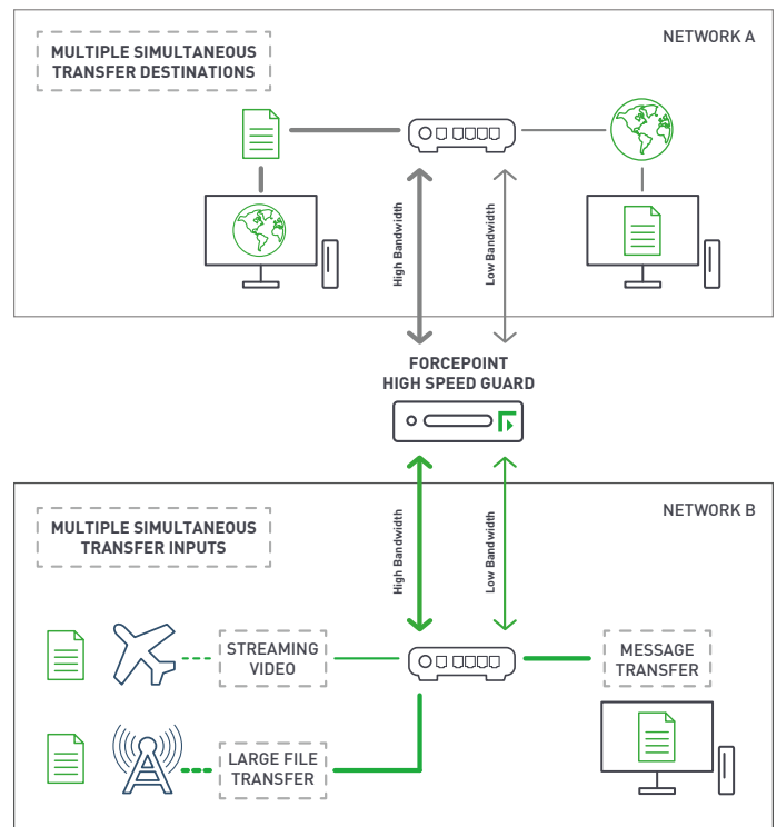
Figure 2. Forcepoint High Speed Guard Simultaneous Transfer Support
