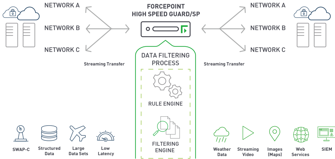
Figure 1. Forcepoint High Speed Guard Architecture
